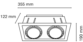
Cut-out 165x327mm
