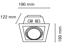
Cut-out 165x165mm
