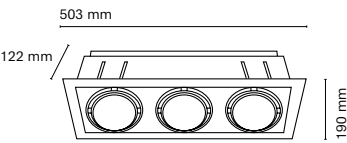
Cut-out 165x472mm
